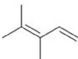
3,4-dimethyl-1,3-pentadiene
