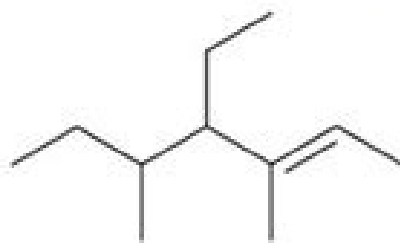
4-ethyl-3,5-dimethyl-2-heptene
