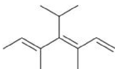
4-isopropyl-3,5-dimethyl-1,3,5-heptatriene
